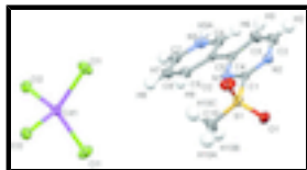
Fig. 1. The structure of the title compound, showing 30% probability displacement ellipsoids and the atom-numbering. Symmetry code for chlorine ions labelled A: -x,y,1/2-z .
