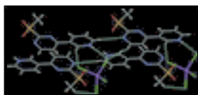
Fig. 3. : The Cd 2 (HL) 4 Cl 8 structural unit, as the result of C—H...Cl hydrogen bonding interactions.
