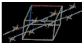
Fig. 2. : One-dimensional chain formed by C7—H7...N2 hydrogen bonding interactions.
